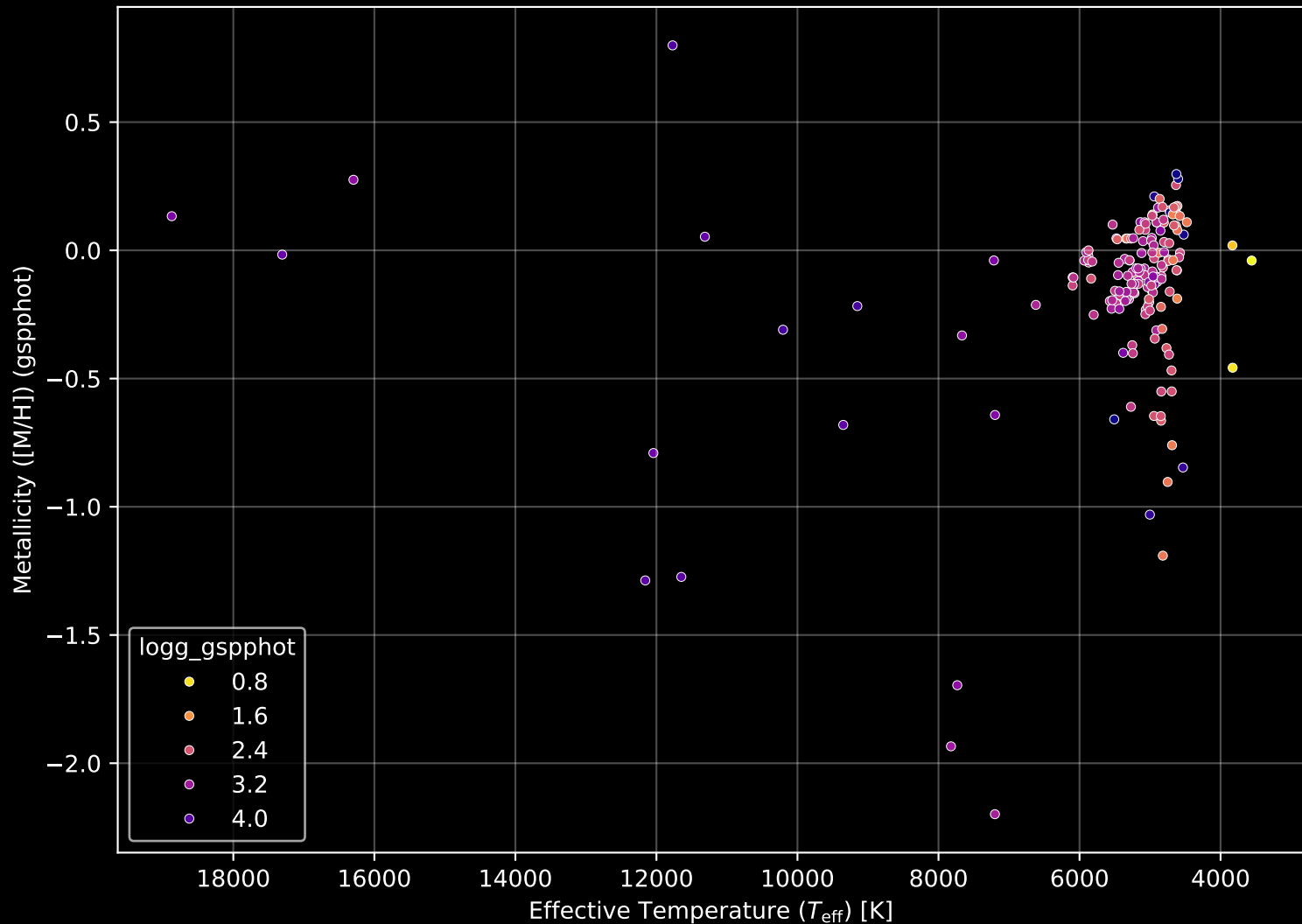
APOGEE DR17 Field: [124-04] Stellar Population Parameters (n= 175)
