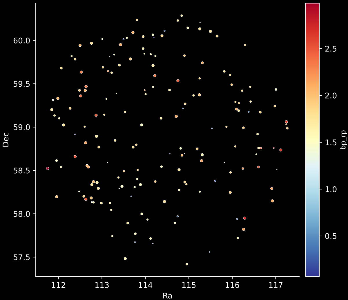
APOGEE DR17 Field: [124-04] Stars: 175
