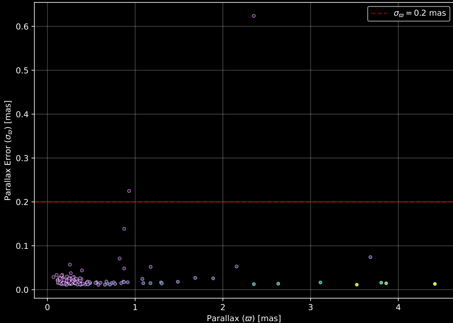
APOGEE DR17 Field: [124-04] Parallax Quality (n= 175)
