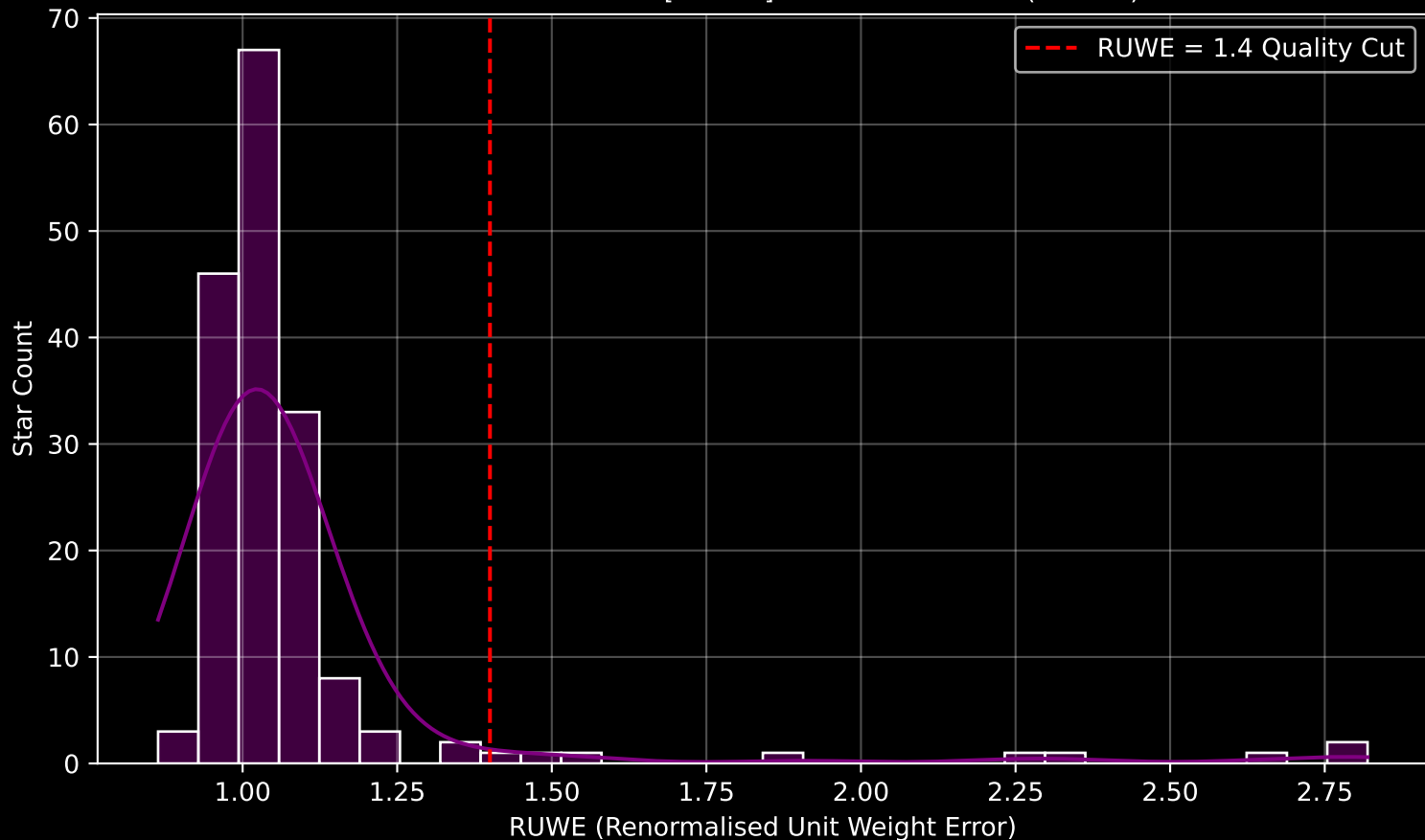
GAPOGEE DR17 Field [124-04] RUWE Distribution (n= 171)
