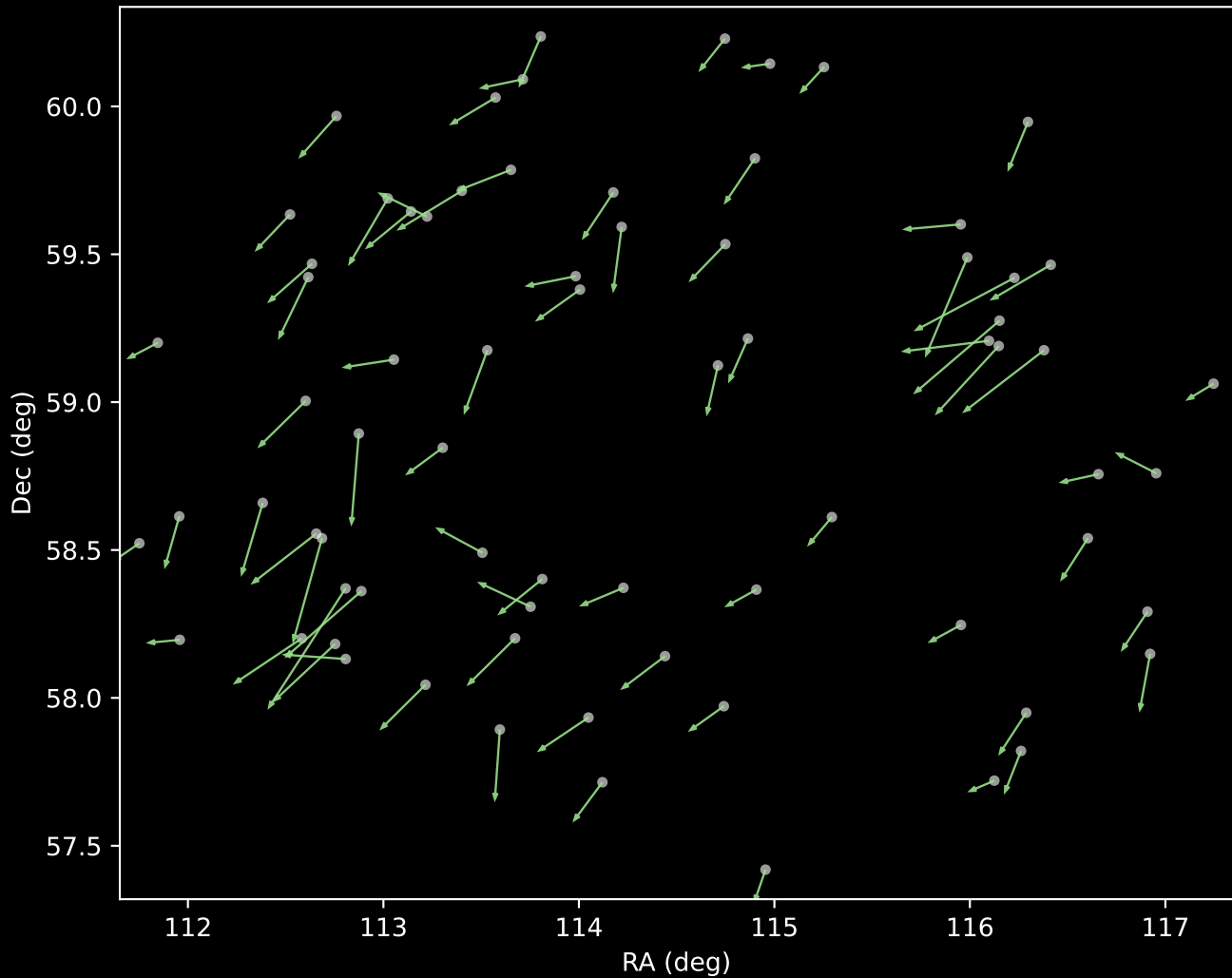
APOGEE DR17 Cluster 5 Proper Motion Vectors (n=73)
