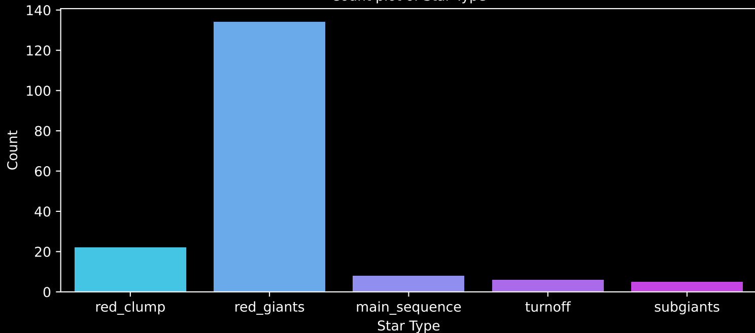
APOGEE DR17 Field: [124-04] Count plot of Star Type
