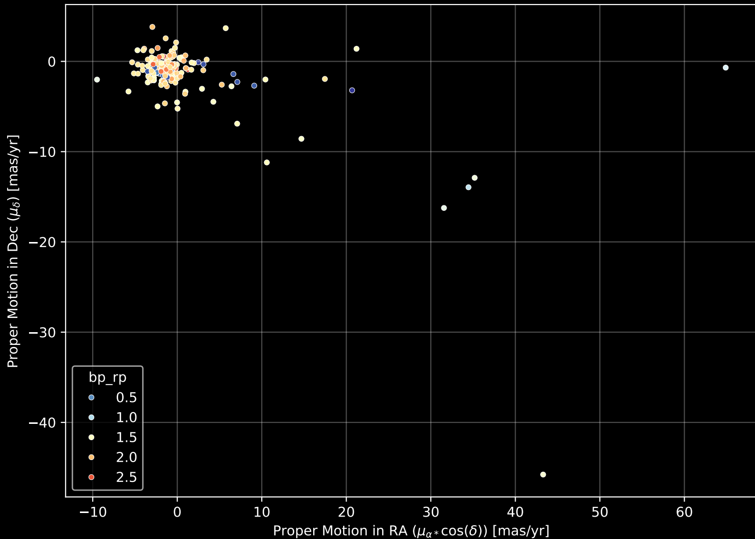
APOGEE DR17 Field: [124-04] Proper Motion Diagram (n= 175)
