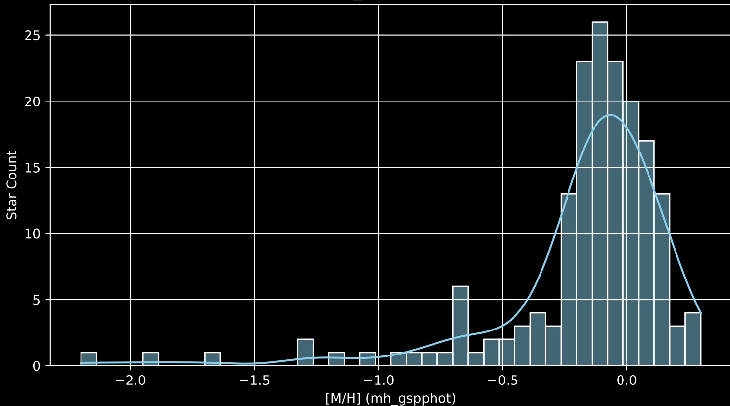
APOGEE DR17 Field: [124-04 [M/H] (mh_gspphot) (n= 174)
